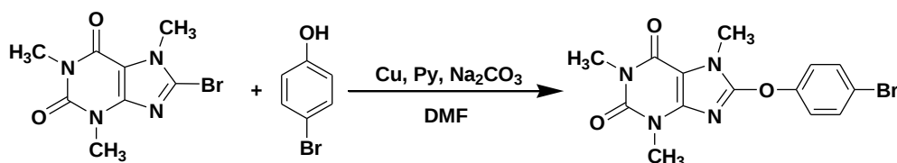
Scheme. 2. Synthetic route for 8-(4'-bromophenoxy) caffeine.
