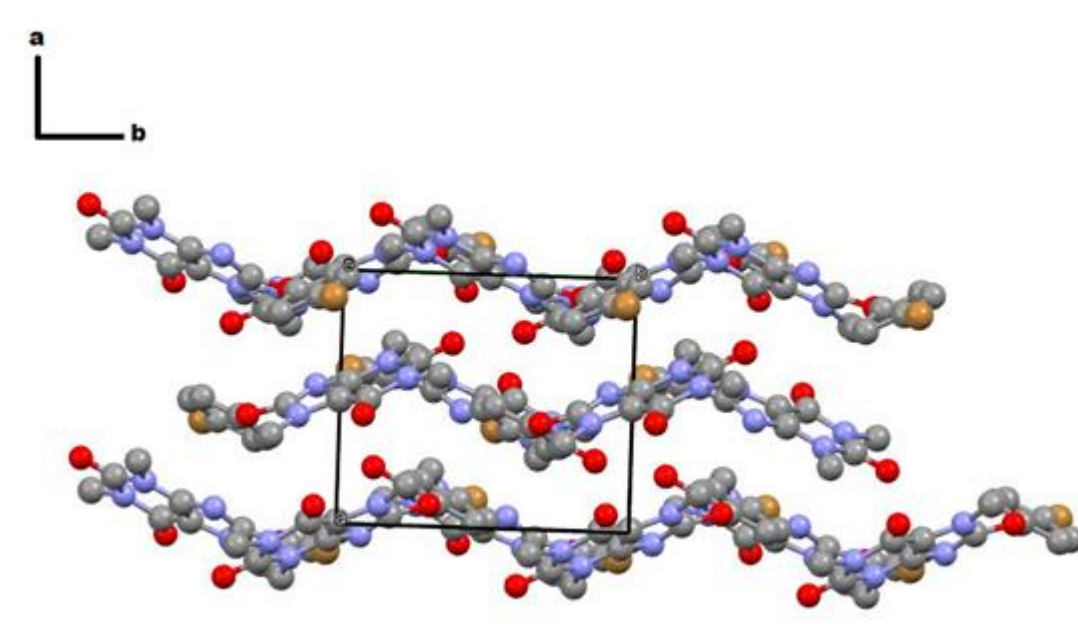
Fig. 2. View of the packing of the BPC molecules along the “c” axis.
