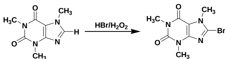
Scheme. 1. Reaction of bromination of caffeine.
